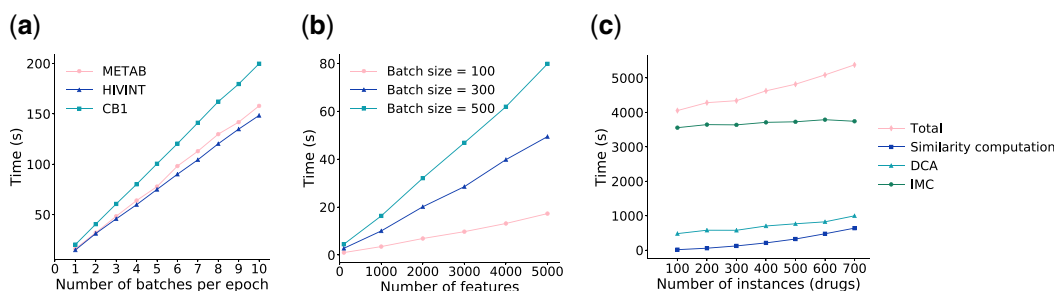
Fig. 3. Scalability of QSARMP and DTIMPC. (a) Running time (in seconds) of training the neural network in QSARMP in one epoch with different numbers of instances (in which the batch size was fixed as 128). The legend represents the different datasets. We used for three datasets as an example from the 15 datasets provided by the Kaggle competition (Ma et al., 2015). The dimensions of input features were 4505, 4306 and 5877 for datasets METAB, HIVINT and CB1, respectively. (b) Running time (in seconds) of training a batch in QSARMP in one iteration with different dimensions of features. We simulated datasets with different dimensions of features by subsampling the features of the original CB1 dataset. (c) Running time (in seconds) of DTIMPC with different numbers of instances (i.e. drugs). We used the simulated data for different numbers of drugs by subsampling the drugs from the original datasets processed in our previous work (Luo et al., 2017). The running time of DTIMPC (with the legend 'Total') consists of the time for three steps, namely, the privacy-preserving pairwise drug–drug similarity computation based on the drug fingerprints and the drug–disease associations (with the legend 'Similarity computation'), the privacy-preserving DCA (with the legend 'DCA') and the privacy-preserving IMC (with the legend 'IMC'). The restart probability of the RWR p_r was fixed as 0.5, the number of expansion terms of Taylor series in the logarithmic operation was fixed as 100, the number of the power method iterations was fixed as 10, the dimension of drug features was fixed as 100, the dimension of protein features was fixed as 400, the number of the IMC iterations was fixed as 5, the latent rank of IMC was fixed as 50 and the number of iterations in updating the decomposed low-rank matrices in IMC was fixed as 200
