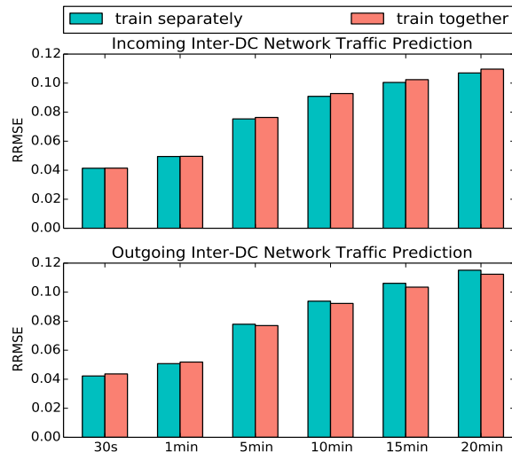
Fig. 9. Prediction errors: combining incoming flows and outgoing flows vs. training separate model for them. We can see that they provide similar results. Giving that the combined model trains faster, we use the combined model
