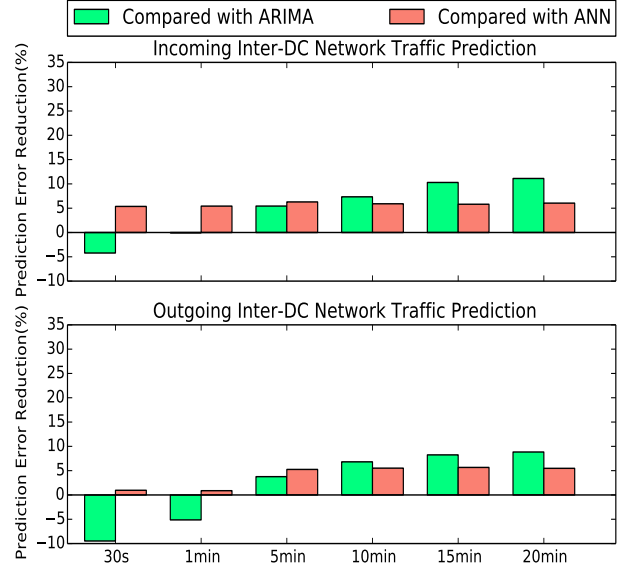
Fig. 11. Prediction errors of the models with elephant flows (but without sublink traffic information).
