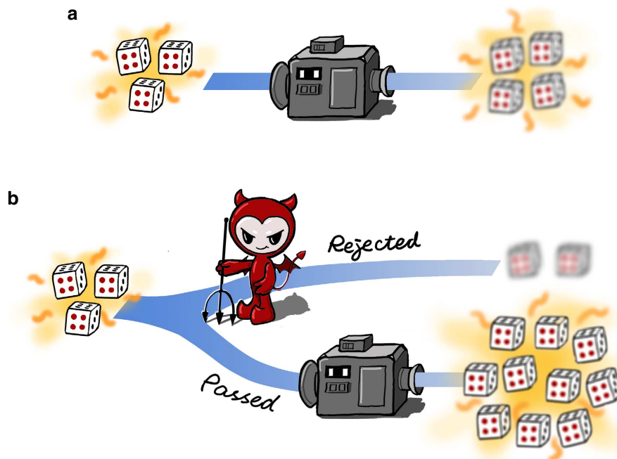
Figure 1 | The advantages of probabilistic super-replication. (a) Every deterministic process is constrained by the SQL: the number of clones that can be produced reliably from N input copies is of order N and the fidelity of the clones cannot approach 1 faster than the inverse of a polynomial of degree 4. (b) Super-replication at the HL: the cloning performances can be dramatically increased by a probabilistic filter, depicted here as a ‘quantum Maxwell demon’ that separates two branches of the wavefunction. In the successful branch, any number of clones of order N^{2-\epsilon} can be produced with fidelity approaching 1 faster than any polynomial.
