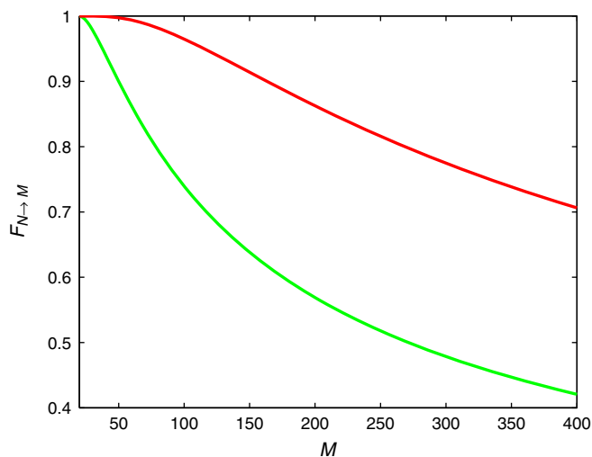
Figure 2 | Replication of linearly polarized photons. The fidelity of the best cloning processes for linearly polarized photons |\psi_t\rangle = \cos t|V\rangle + \sin t|H\rangle is plotted here for N=20 input copies, with the number M of output clones ranging from 20 to 400. The red (green) line refers to optimal cloning with (without) filter.
