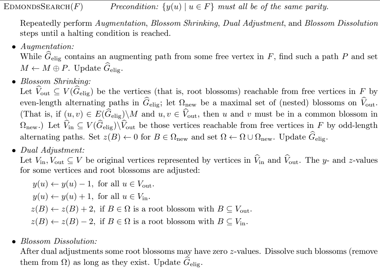
Figure 2: A generic implementation of Edmonds' search procedure. Data structural issues are ignored, as is the eligibility criterion, which determines \widehat{G}_{\text{elig}} .
