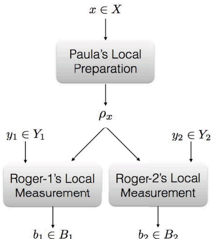
FIG. 2: Paula, Roger-1, and Roger-2 in a three-party prepare-and-distribute experiment.
