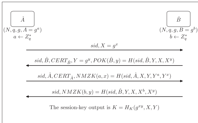
Fig. 1. Deniable Internet key-exchange (the main mode).
