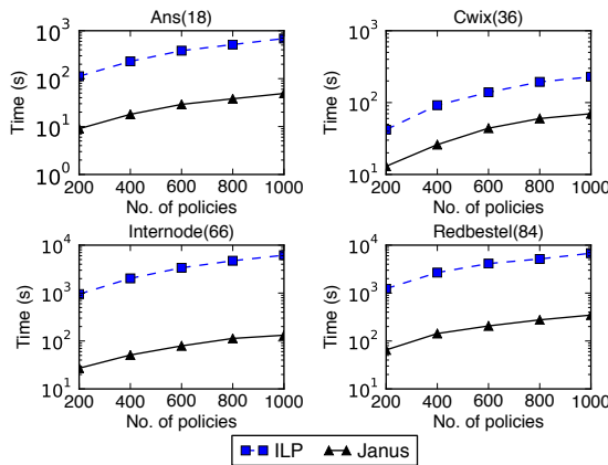
Figure 11: JANUS VS ILP with varying the number of policies in the network. Each policy has 20 endpoints
