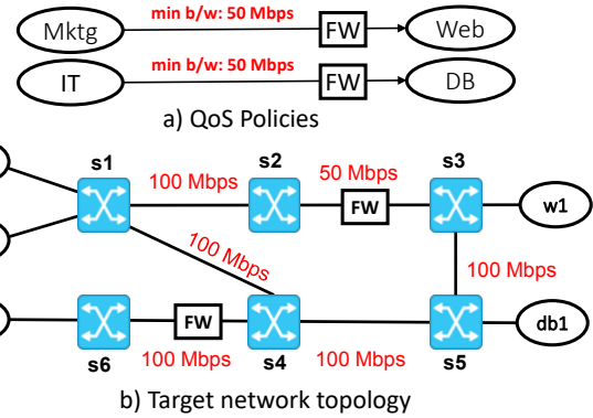
Figure 2: Example of policies contending for network resources. Endpoints m1 & m2 belong to Marketing group, it1 to IT, db1 to DB and w1 to Web
