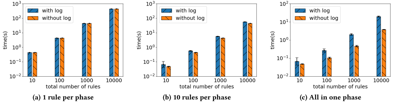
Figure 4: Overhead Measurement
