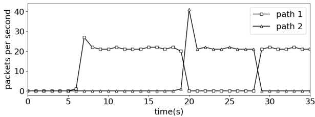
Figure 3: Failure recovery
