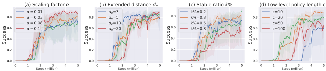
Figure 9: Ablation studies of hyper-parameter selection in the Ant Push (Images) task.
